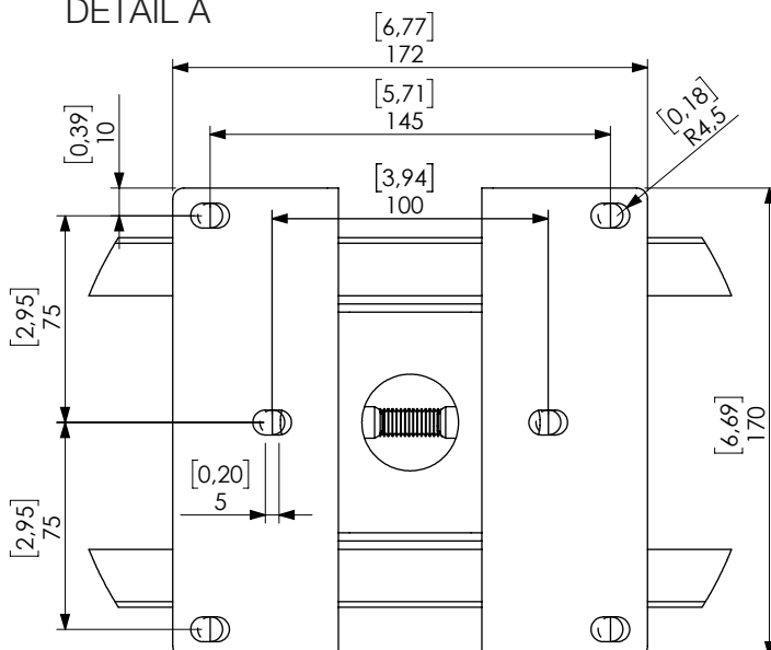
DETAIL A
