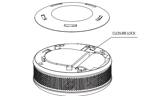
Fig. 3 - Fibaro Smoke Sensor bottom view with the battery installed
