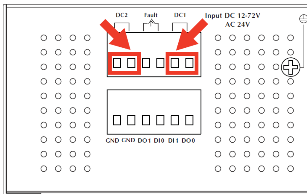
Figure 2-17: IGS-12040MT Upper Panel
