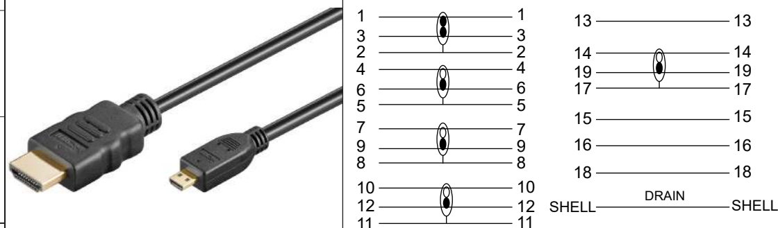
PIN-Belegung / PIN Assignment
